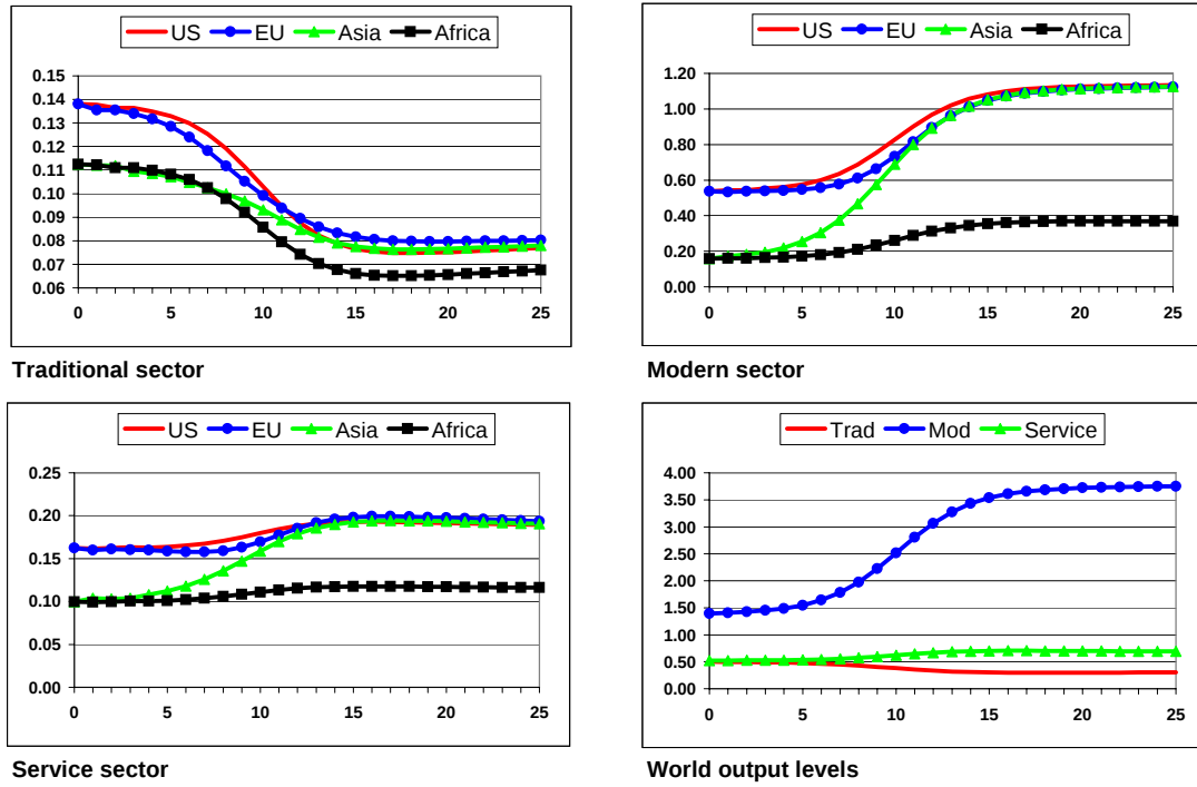
Figure 4.4: Output dynamics
