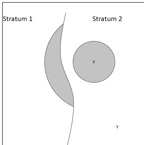
Figure 4.2: Grey shading indicates the set of all points that, if they were selected, would lead to the selection of household X.
