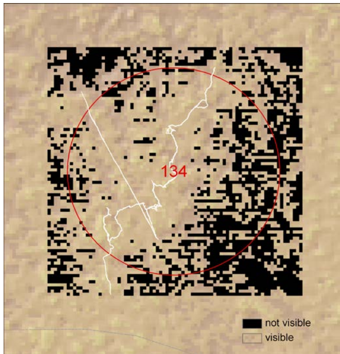
Figure 5. Viewshed Analysis
