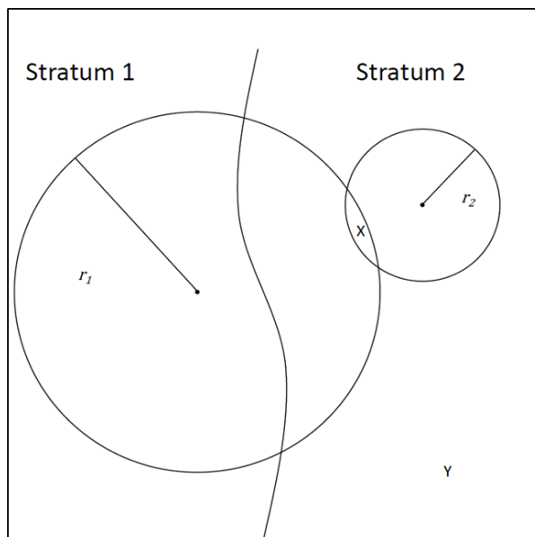
Figure 4.1: Household X, in stratum 2, can be selected by points selected from stratum 1 or 2. r_1 is the selection radius used in stratum 1; r_2 is the selection radius in stratum 2.
