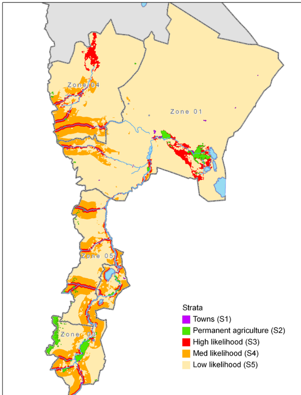
Figure 2: Stratification Map
