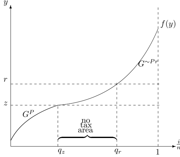
Figure 3: Progressive Transfers, setting a richness line
