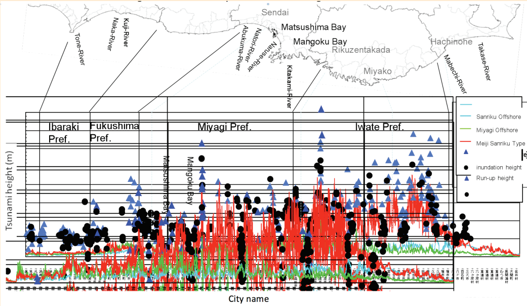
FIGURE 5: Actual versus predicted tsunami height
