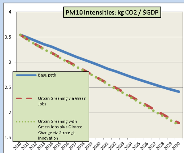
Figure 6.5 PM10 intensities
