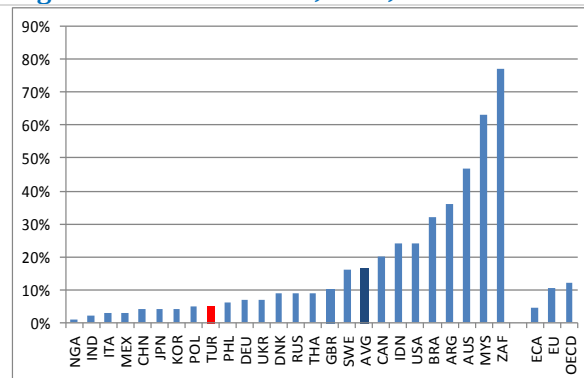
Figure 2.15 Forest loss, 2010, %
