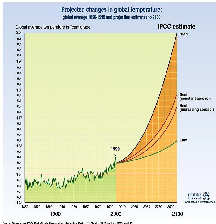
Figure 1- Predicted changes in global temperature
