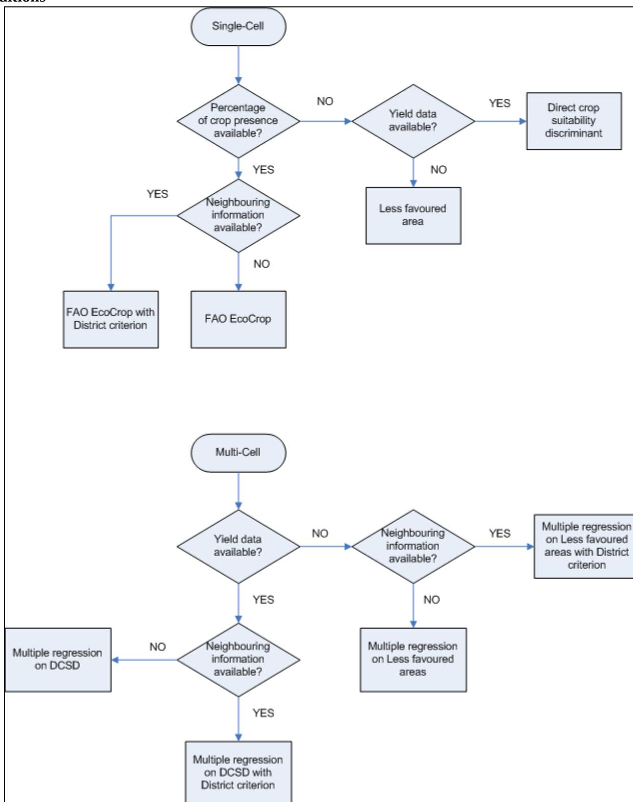
Figure I20. Flow chart of the logic behind the UNIMI.Suitability feature for automatically selecting the most suitable approach according to the availability of data under specific conditions
