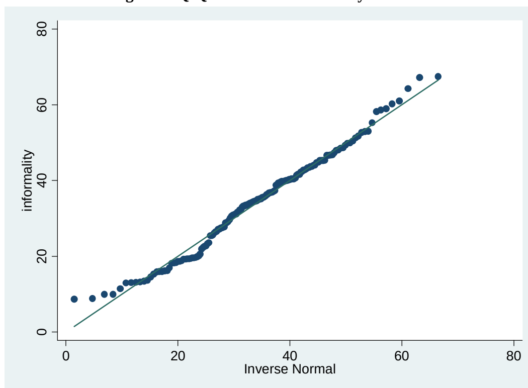
Figure 2. Q-Q Plot of the Informality Measure
