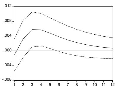
Figure 2: Impulse-Response Functions
