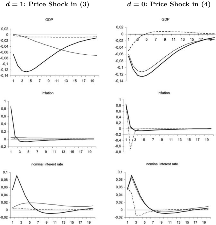
Figure 2. Impulse Response to a Price Shock in the 20-Quarter Taylor Model for Different Specifications of the Price Shock (Baseline Parameters)
