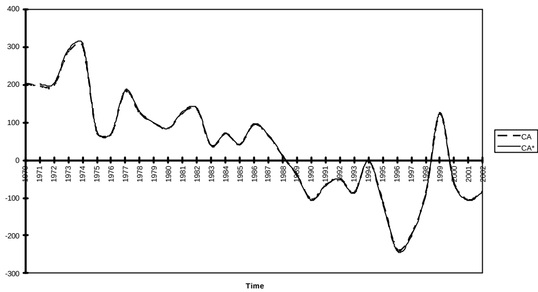
Fig 2.3a: Malaysia --- Optimal and Actual Current Account.
